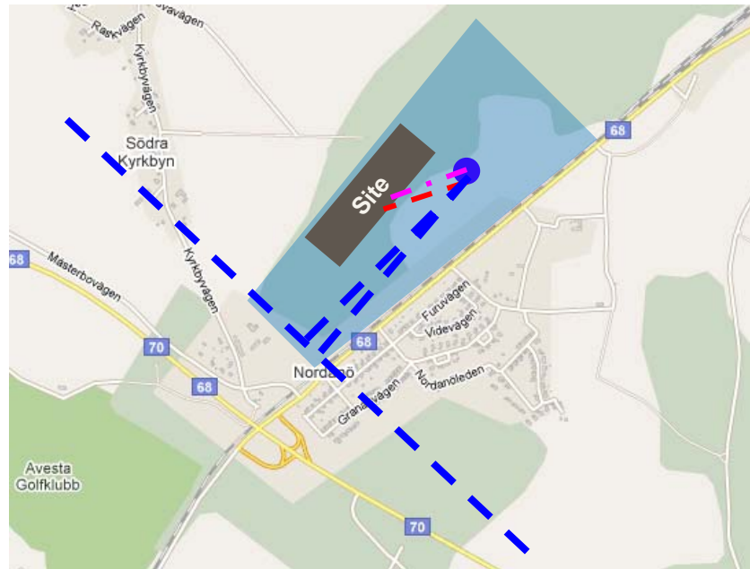
Power alternative II, 40 MW
